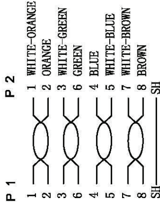
WIRING DIAGRAM
